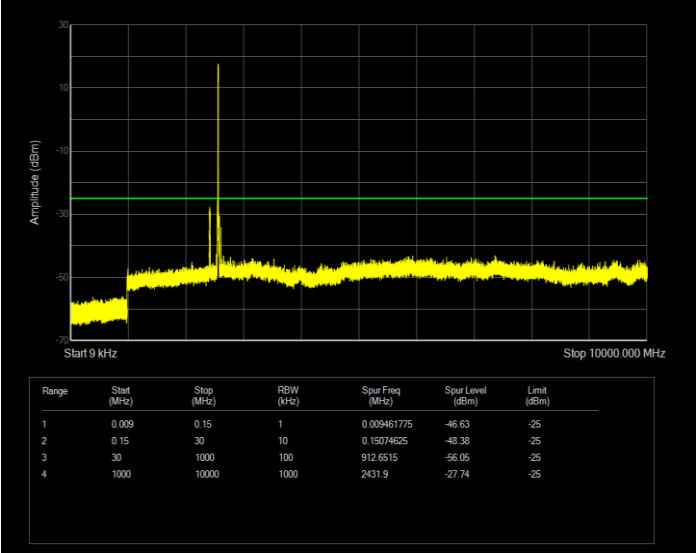
Band38 QAM16 BW=10MHz Channel=38000 RB Size=50 Position=#0
