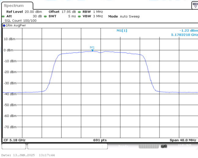
11AC20MIMO-Ant1-5180-PASS
