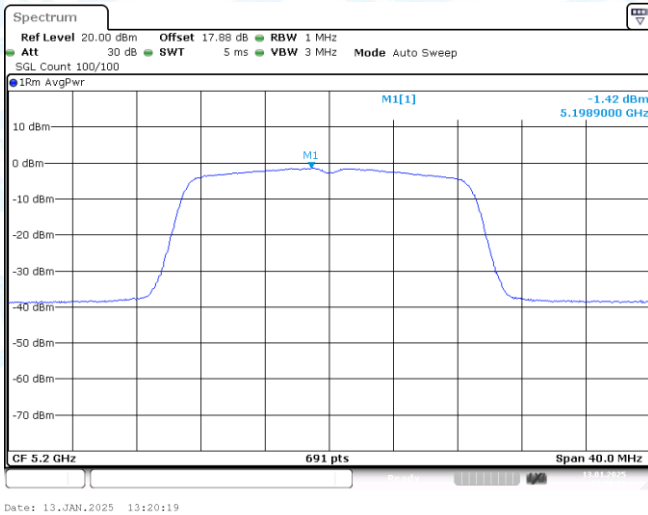
11AC20MIMO-Ant1-5200-PASS
