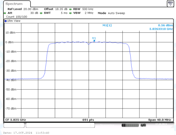
11AX20MIMO-Ant2-5825-PASS
