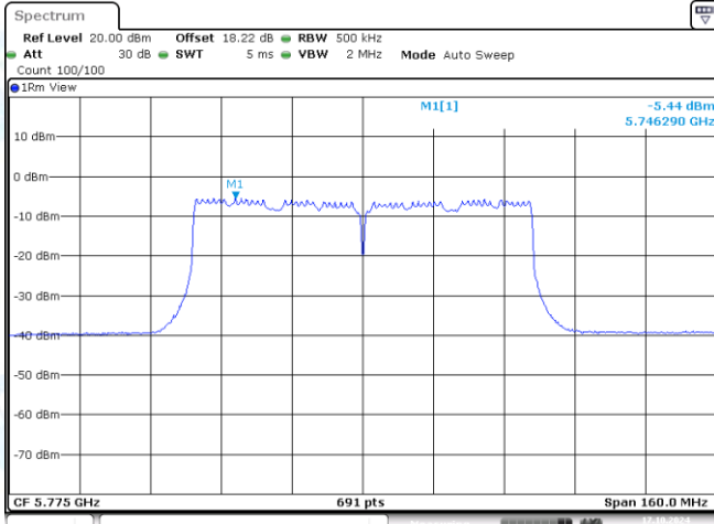
11AC80MIMO-Ant1-5775-PASS
