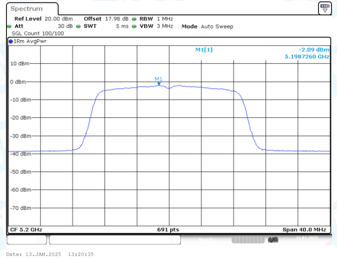
11AC20MIMO-Ant2-5200-PASS
