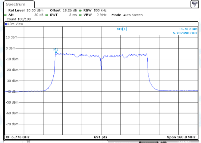
11AC80MIMO-Ant2-5775-PASS
