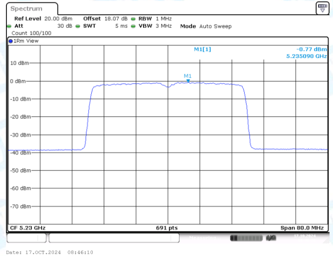
11AX40MIMO-Ant2-5230-PASS
