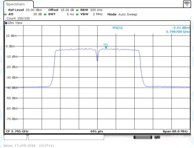
11N40MIMO-Ant2-5795-PASS
