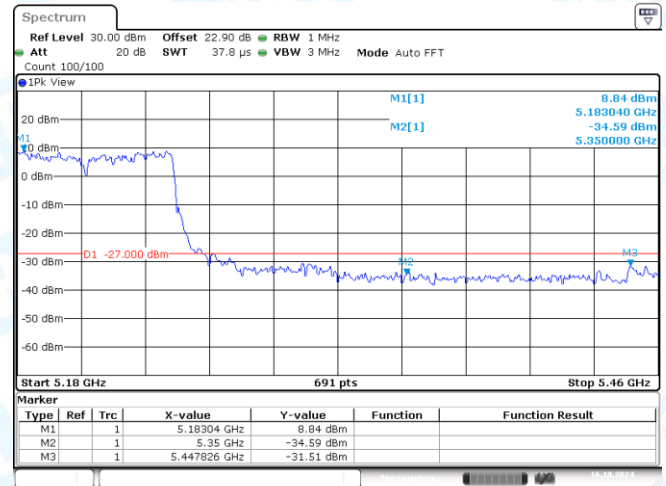
11AC80MIMO-Ant1-5210-PASS
