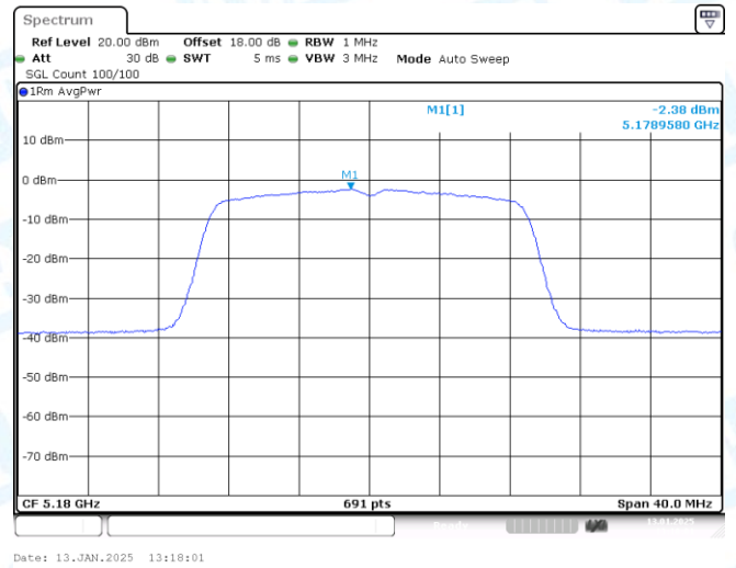
11AC20MIMO-Ant2-5180-PASS
