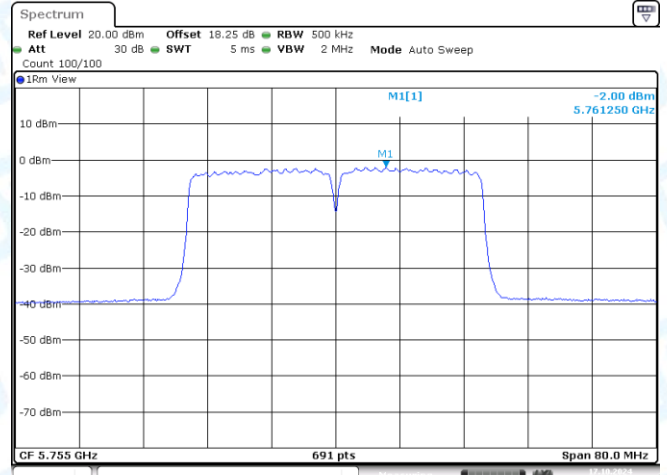
11AC40MIMO-Ant2-5755-PASS
