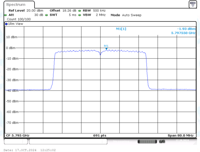
11AX40MIMO-Ant2-5795-PASS
