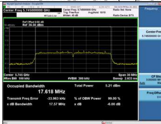
-6dB Emission Bandwidth 5_8WiFi 802_11ac(VHT20)_5745_20M
