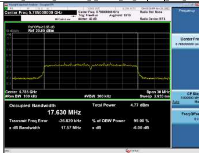
-6dB Emission Bandwidth 5_8WiFi 802_11n(HT20) 5785_20M
