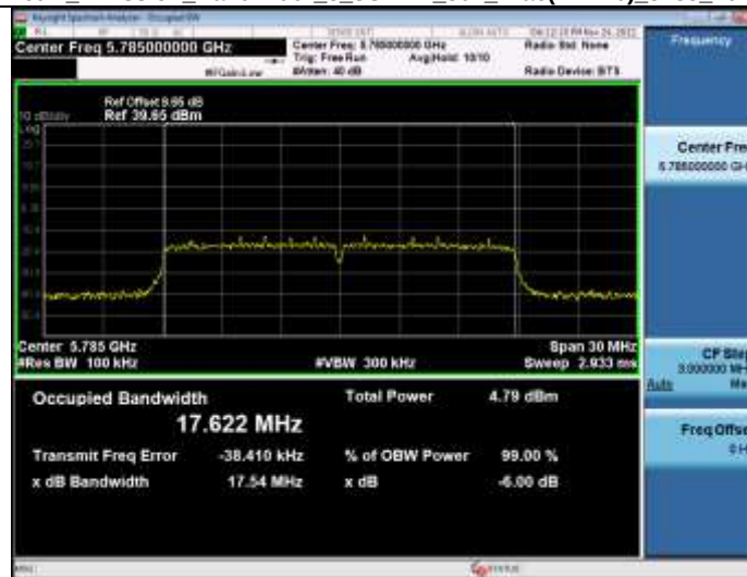
-6dB Emission Bandwidth 5_8WiFi 802_11ac(VHT20)_5785_20M
