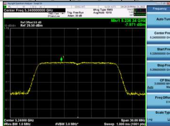
Power Spectral Density 5_2WiFi 802_11n(HT20) 5240_20M
