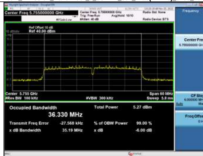
-6dB Emission Bandwidth 5_8WiFi 802_11ac(VHT40)_5755_40M
