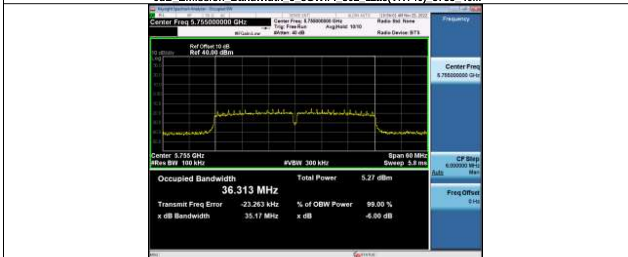
-6dB Emission Bandwidth 5.8GHz WiFi 802.11ac(VHT40) 5755 40M
