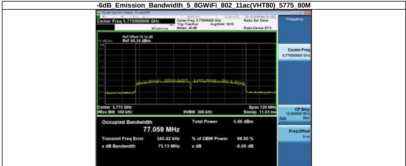
-6dB Emission Bandwidth 5 802.11ac(VHT80) 5775_80M
