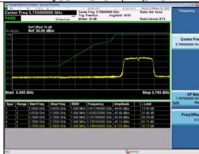
Bandedge 5_8WiFi_802_11ac(VHT40)_5755_40M
