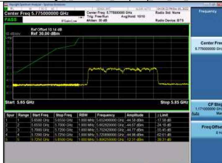
Bandedge_5_8GWiFi_802_11ax(HE80)_5775_80M_up
