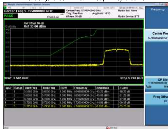
Bandedge 5_8WiFi_802_11ac(VHT40)_5755_40M
