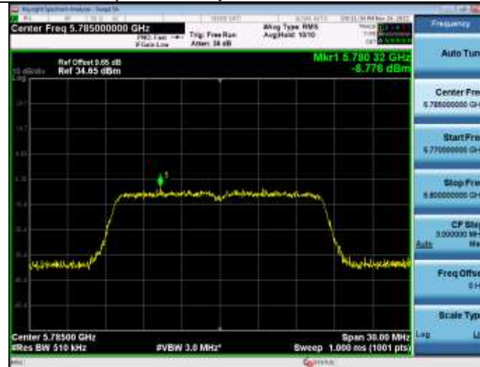
Power Spectral Density 5_8WiFi 802_11a 5785 20M
