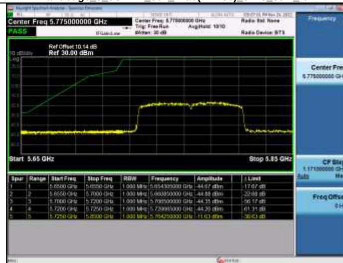
Bandedge 5 8WiFi 802 11ac(VHT80) 5775_80M_up
