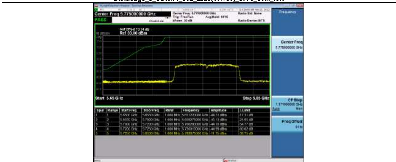
Bandedge 5 8WiFi 802 11ac(VHT80) 5775_80M_up
