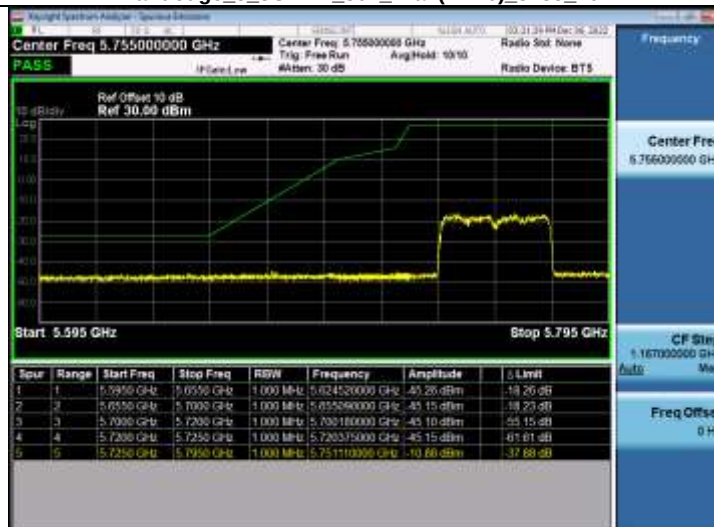
Bandedge 5_8WiFi_802_11ax(HE40)_5755_40M
