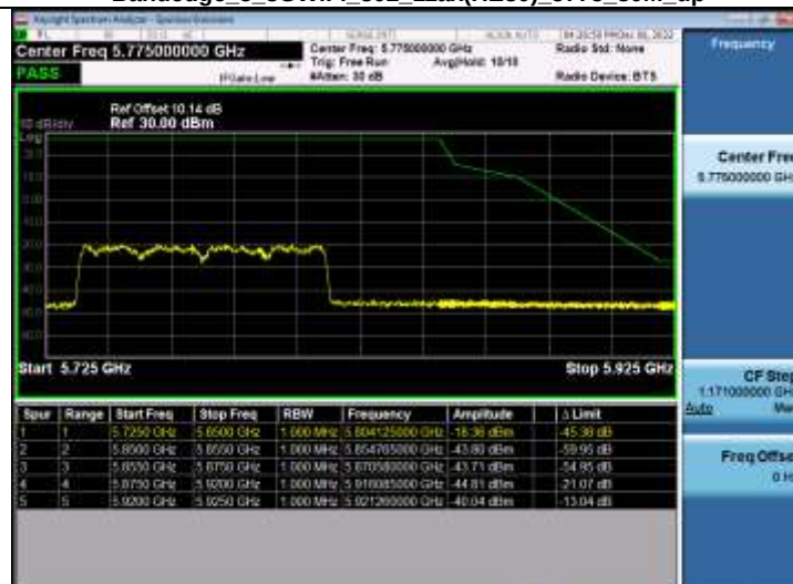
Bandedge 5_8WiFi_802_11ax(HE80)_5775_80M_up
