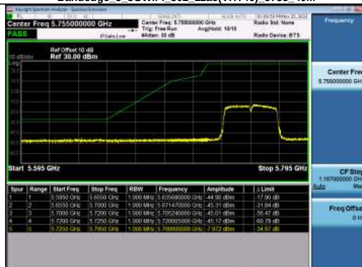
Bandedge 5_8WiFi_802_11ac(VHT40)_5755_40M
