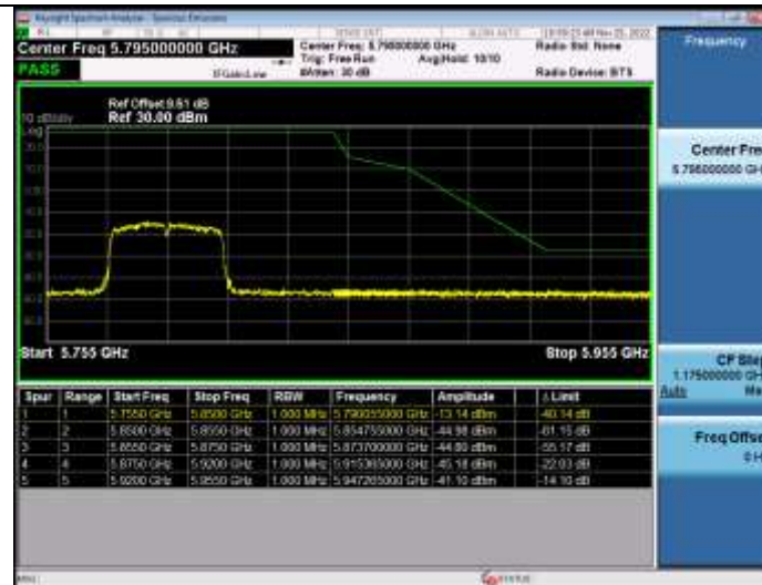
Bandedge 5 8WiFi 802 11ac(VHT80) 5775_80M_low
