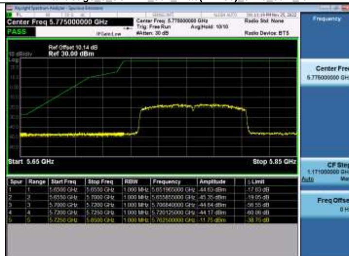
Bandedge_5_8WiFi_802_11ac(VHT80)_5775_80M_up
