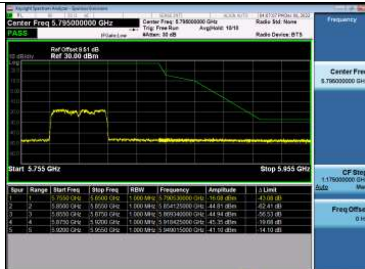
Bandedge_5_8GWiFi_802_11ax(HE80)_5775_80M_low
