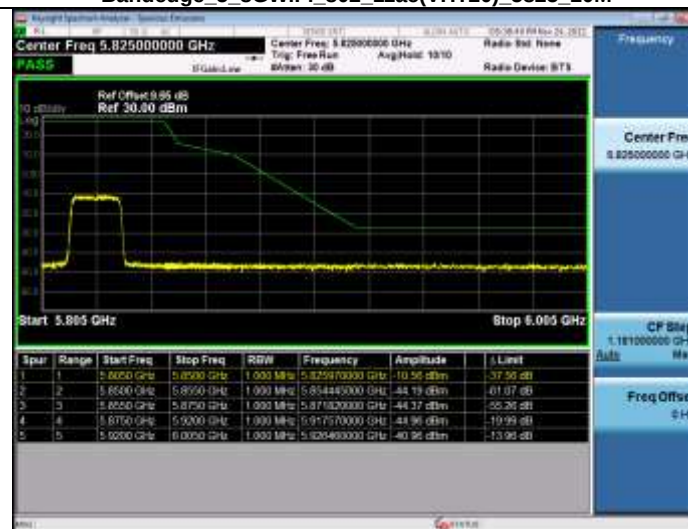
Bandedge 5_8WiFi_802_11ac(VHT20)_5825_20M
