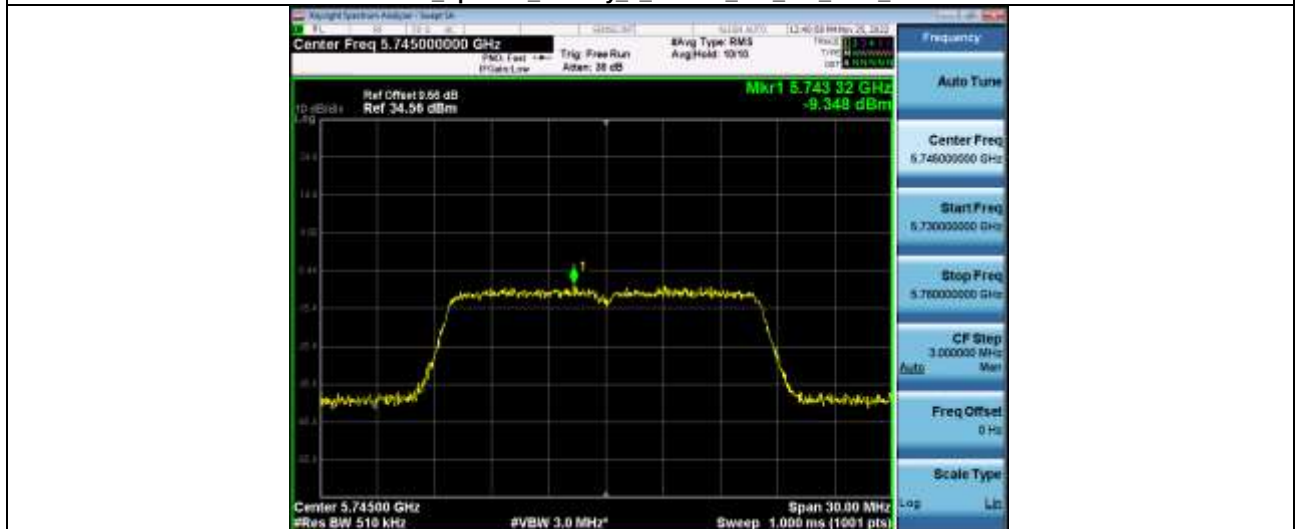
Power Spectral Density 5_8WiFi 802_11a 5745_20M
