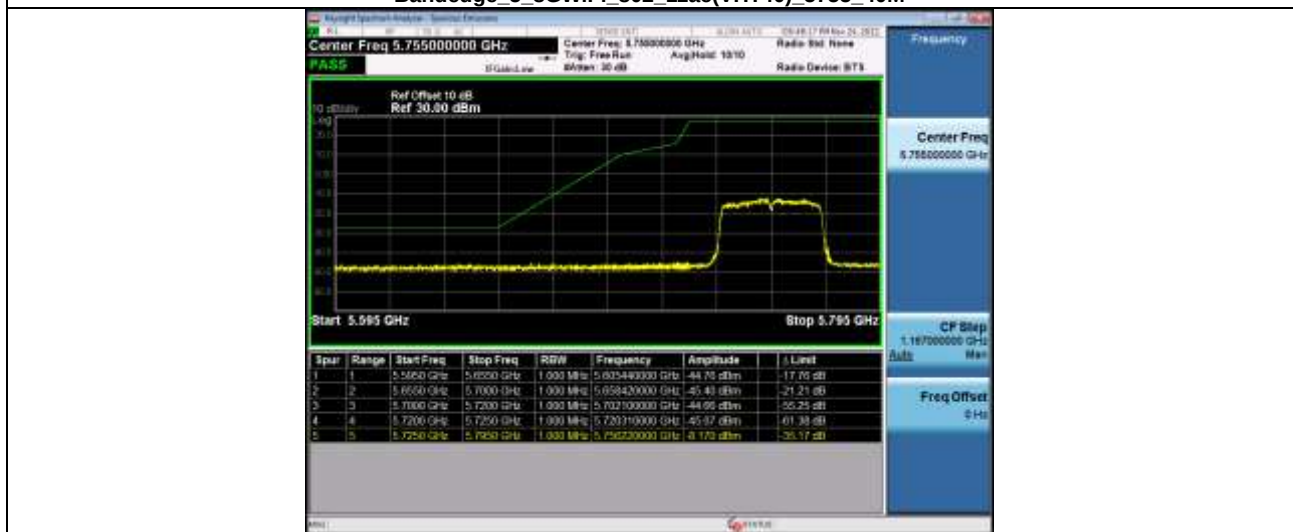
Bandedge 5_8WiFi_802_11ac(VHT40)_5795_40M
