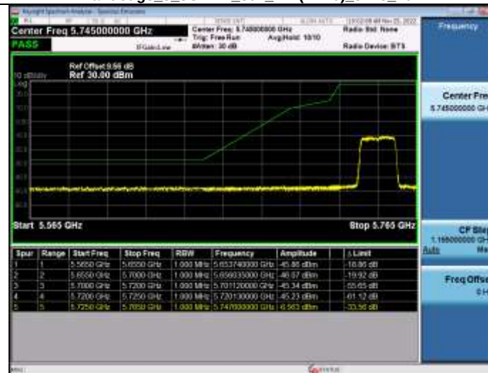
Bandedge 5 8WiFi 802_11n(HT20) 5745_20M
