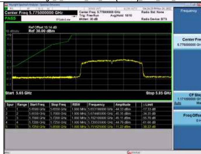
Bandedge_5_8WiFi_802_11ac(VHT80)_5775_80M_up
