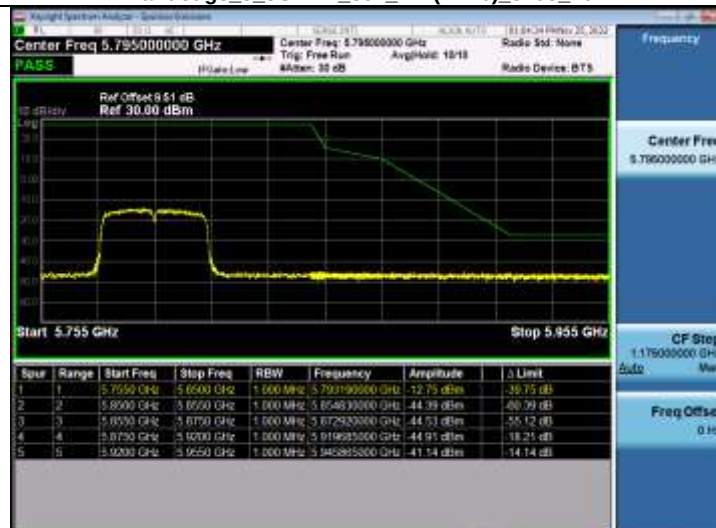
Bandedge 5_8WiFi_802_11n(HT40)_5795_40M
