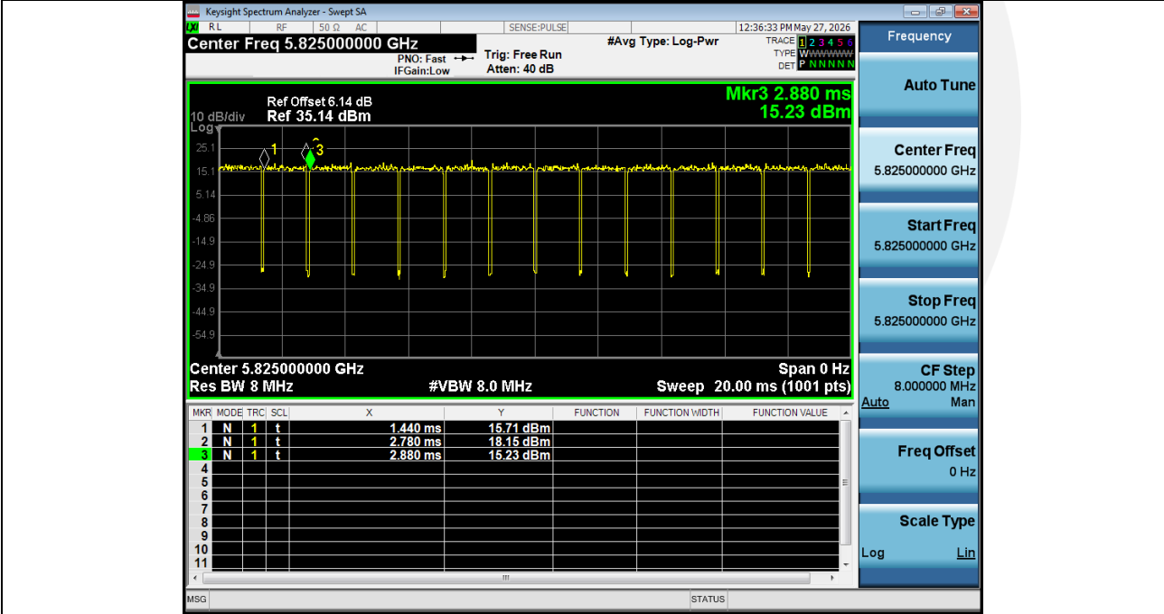
Duty_Cycle_NVNT_ANT1_802_11n(HT20)_5825
