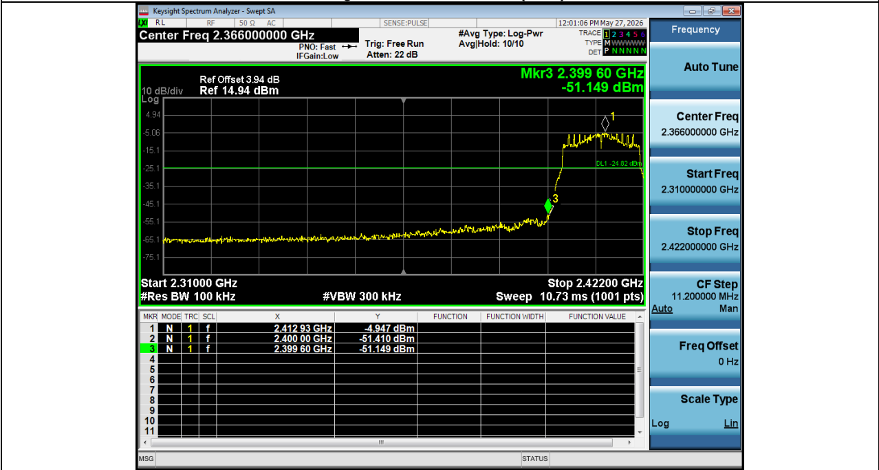
2_Bandedge_NVNT_ANT1_802_11n(HT20)_2412
