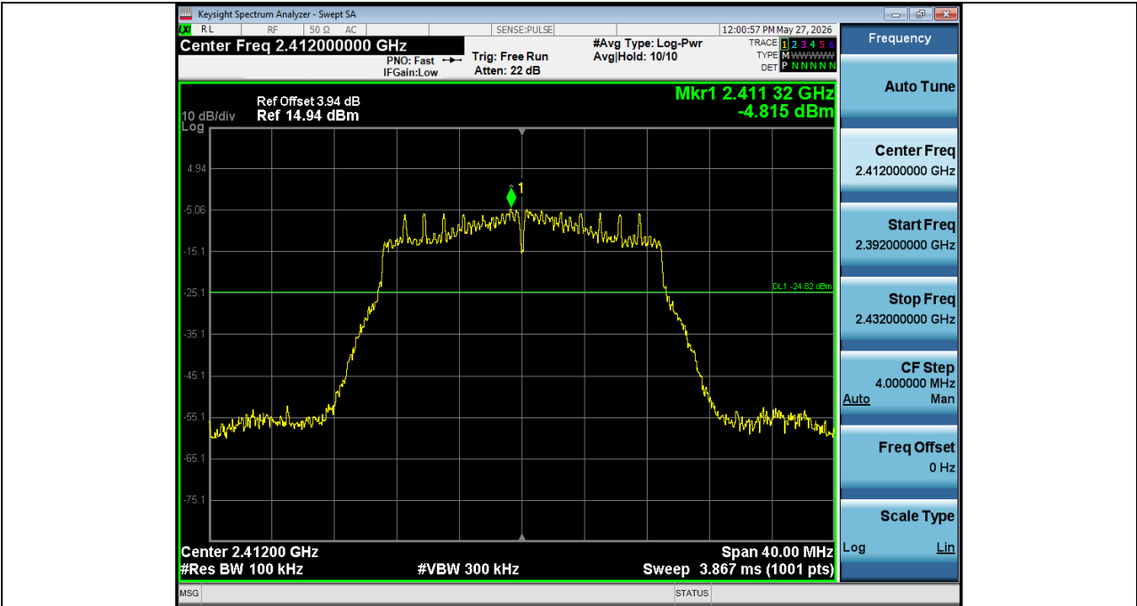
2_Bandedge_NVNT_ANT1_802_11n(HT20)_2412
