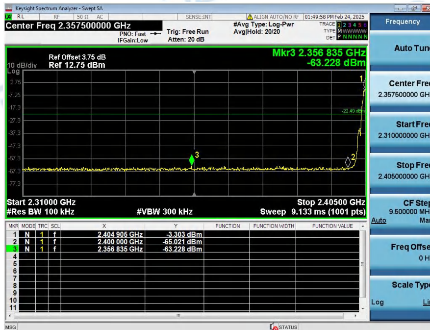
2_Bandedge_NVNT_ANT1_1Mbps_2405
