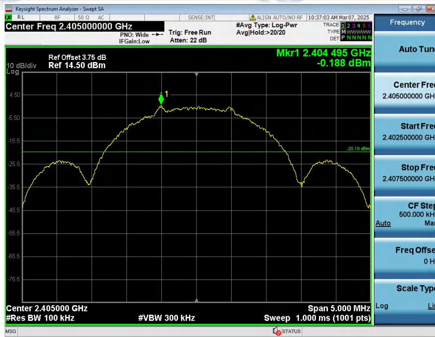
2_Bandedge_NVNT_ANT1_1Mbps_2405
