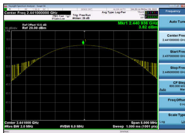
Output Power: 8DPSK,2441MHz,3DH5
