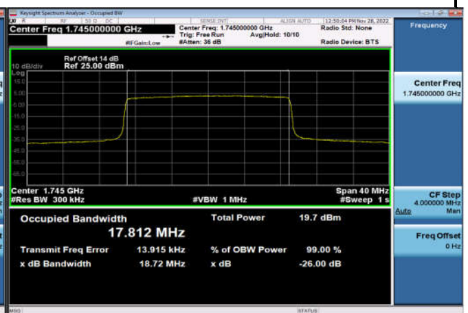
FDD66_MidRange_20MHz_1745MHz_Q16
