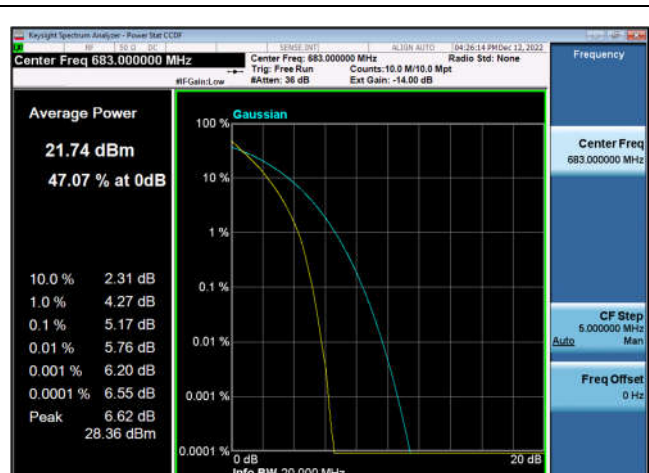
FDD71_MidRange_20MHz_683_OneRB _high_Q16
