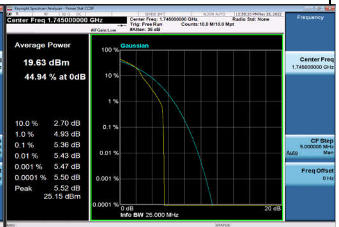
FDD66_MidRange_20MHz_1745_OneRB _high_Q16
