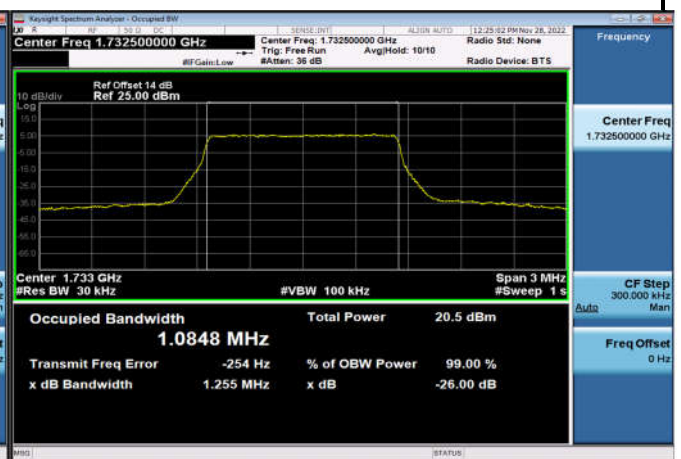
FDD04_MidRange_3MHz_1732.5MHz_Q16
