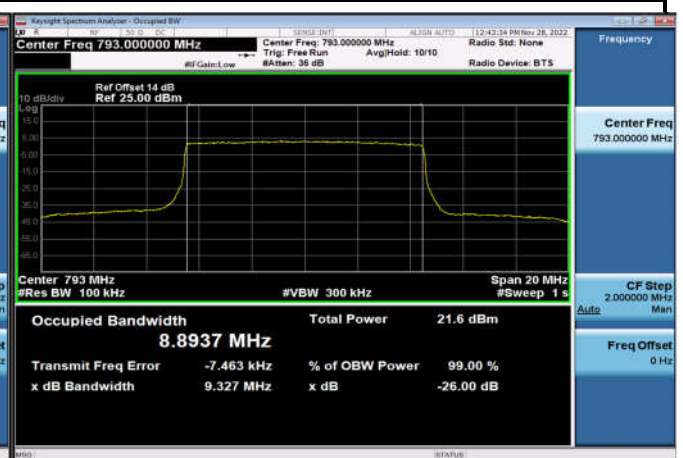
FDD14_MidRange_10MHz_793MHz_Q16
