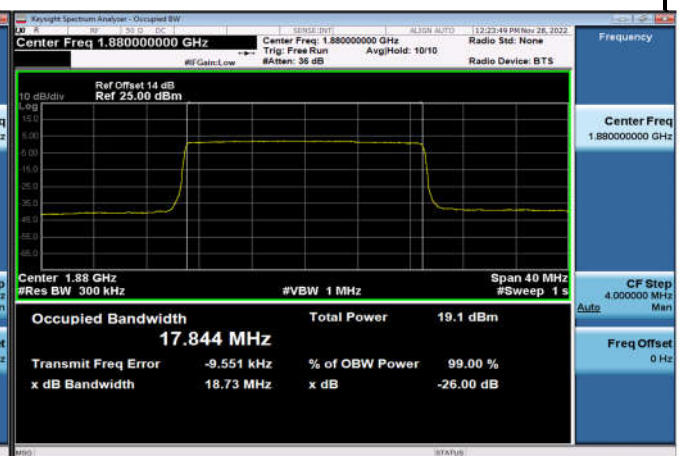
FDD02_MidRange_20MHz_1880MHz_Q16
