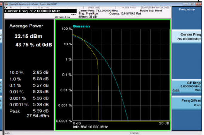
FDD13_LowRange_10MHz_782_OneRB _high_Q16
