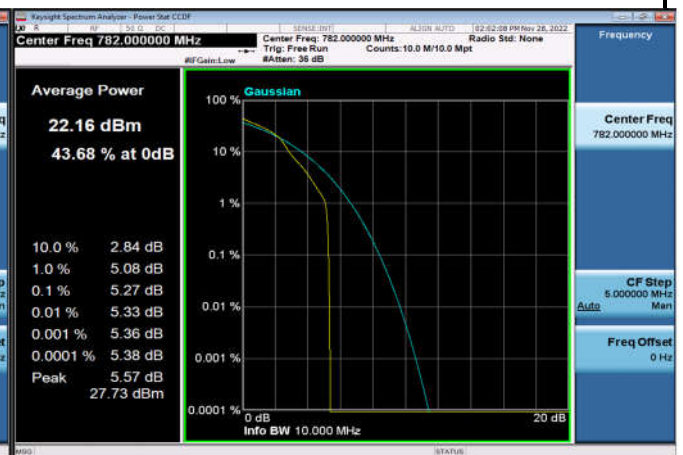
FDD13_MidRange_10MHz_782_OneRB _high_Q16
