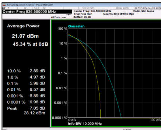
FDD05_MidRange_10MHz_836.5_fullIRB _Q16
