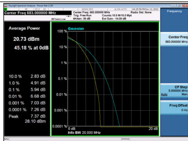
FDD71_MidRange_20MHz_683_fullIRB _Q16
