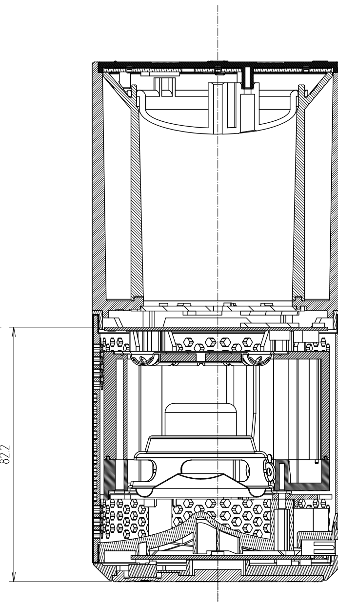
SECTION B-B
