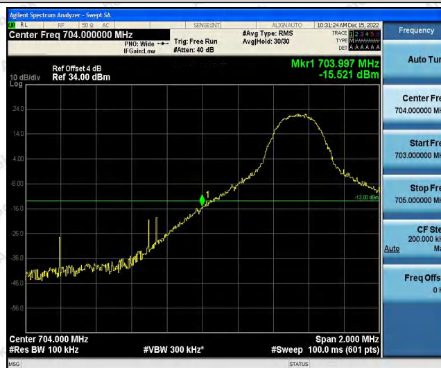
Band17-5MHz-16QAM-23755-1RB#24
