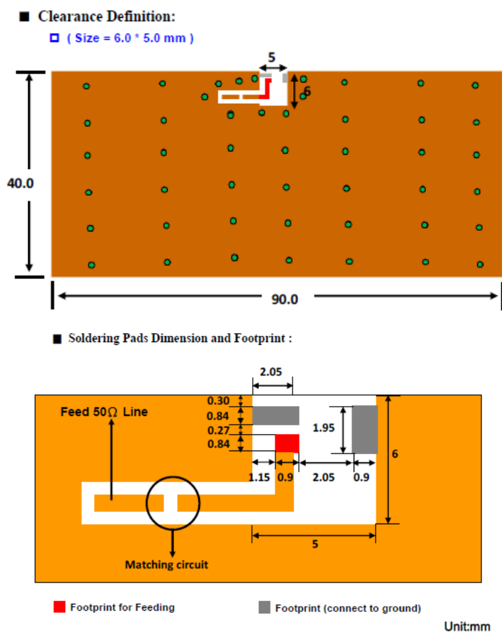
Fig. 2 Outlook and dimension of evaluation board
