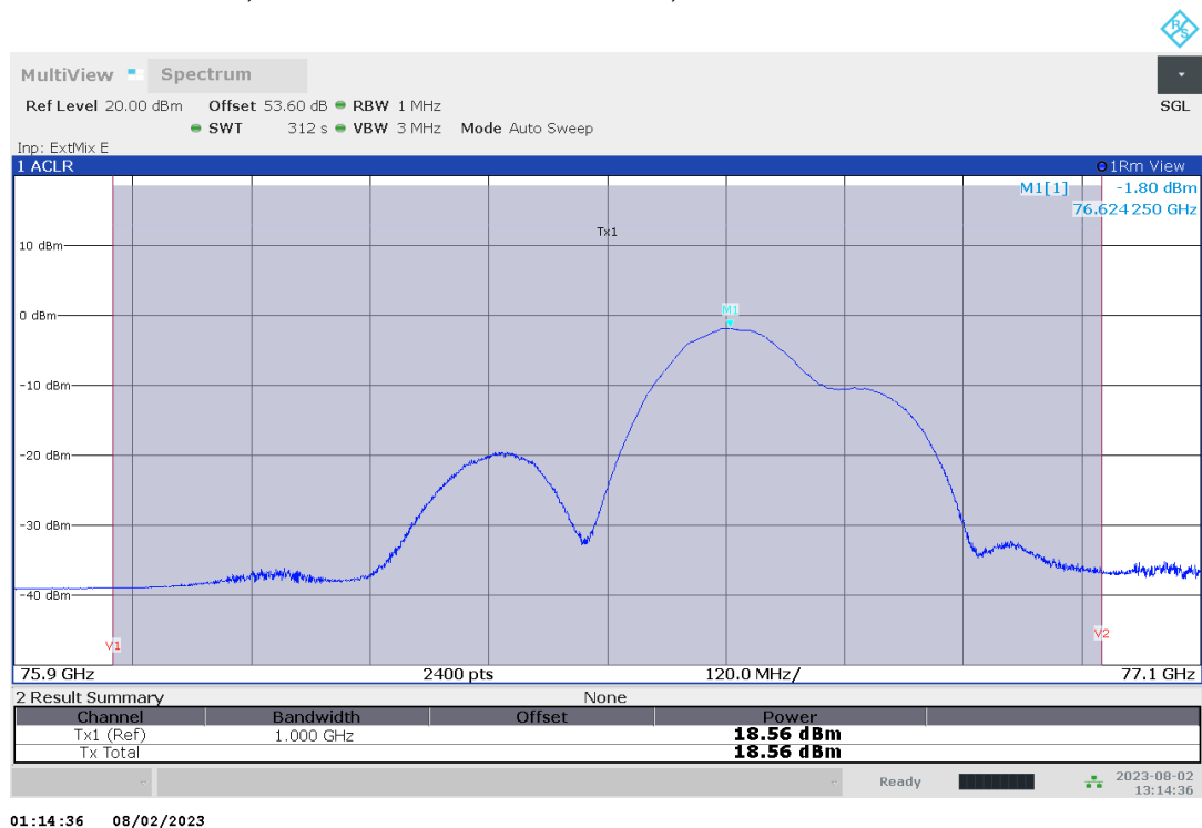
Plot no. 2: Mean Power EIRP, RMS detector / Channel Power, Front mode
