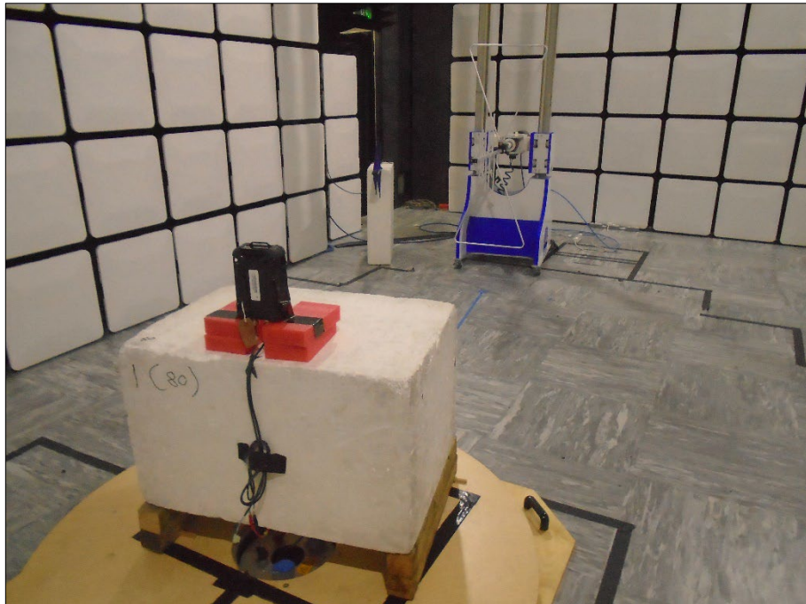
Figure 3 – Radiated Emissions Lab Testing (30 MHz to 1 GHz)
