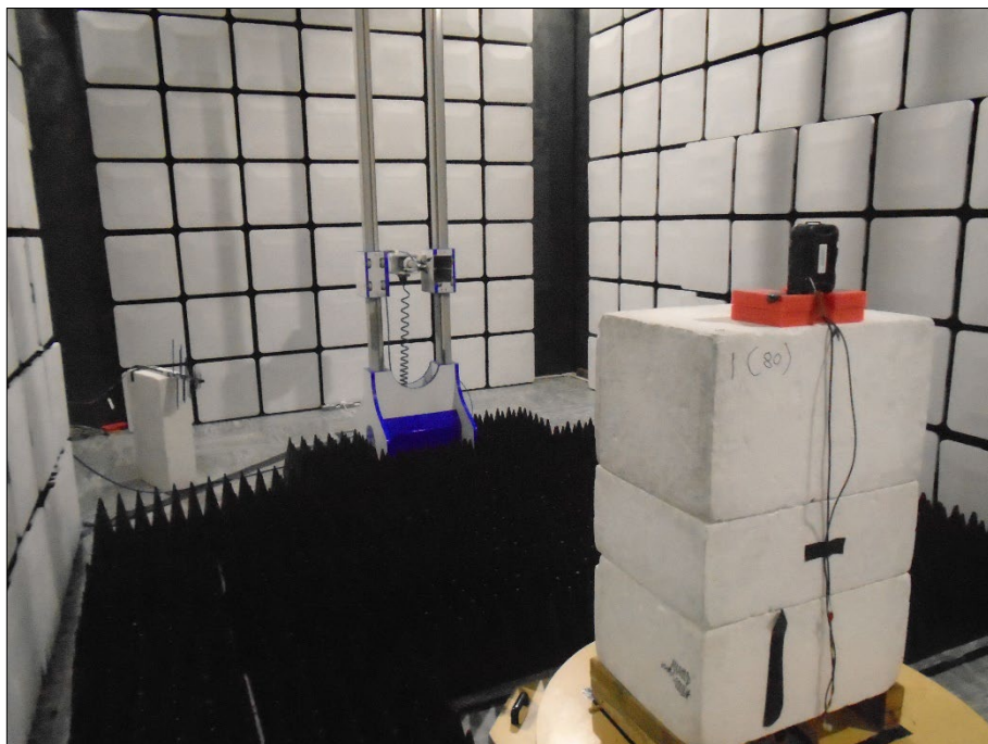
Figure 4 - Radiated Emissions Lab Testing (1 GHz to 10 GHz)
