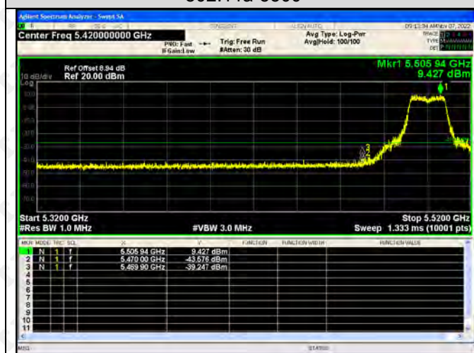
802.11ac(VH20)-5500
