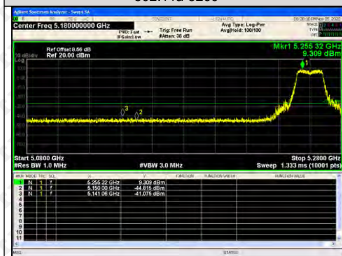
802.11ac(VH20)-5260
