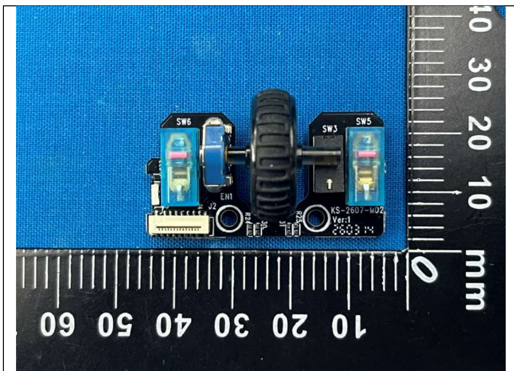
Mechanical switch
