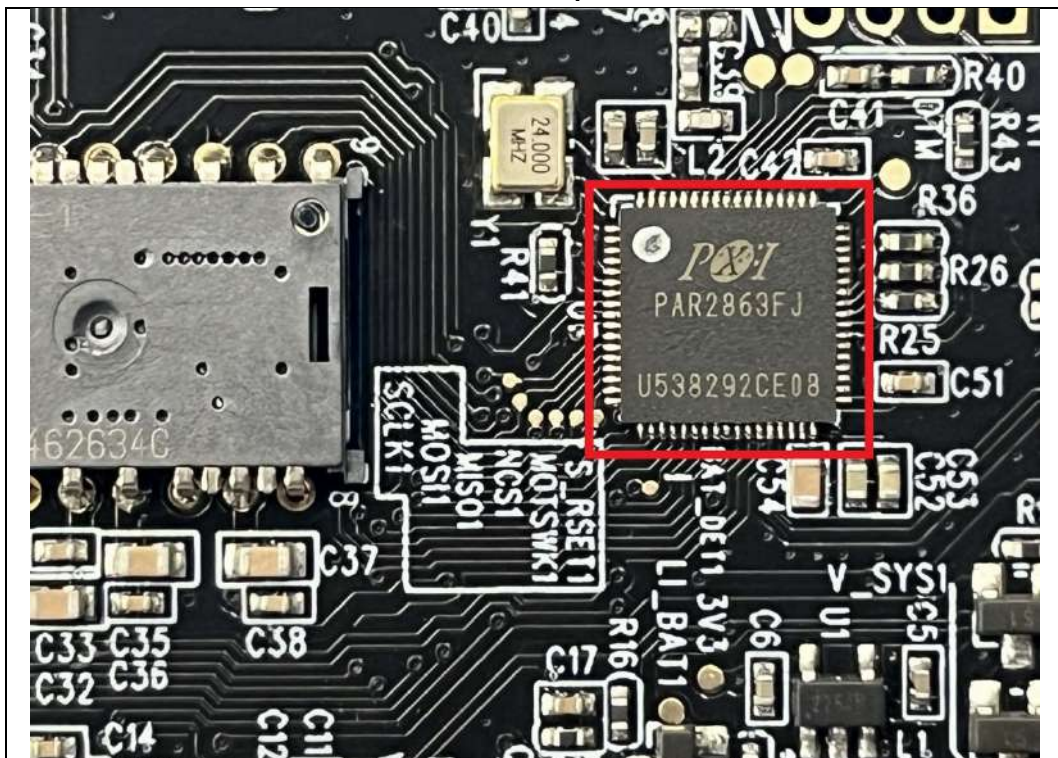
RF Chip
