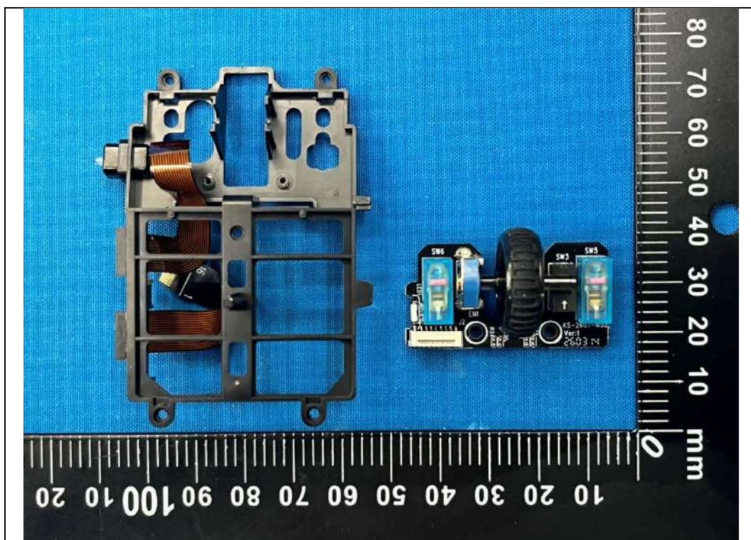
Mechanical switch
