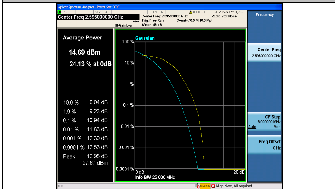
Band38-5MHz-16QAM-38000-25RB#0-PASS
