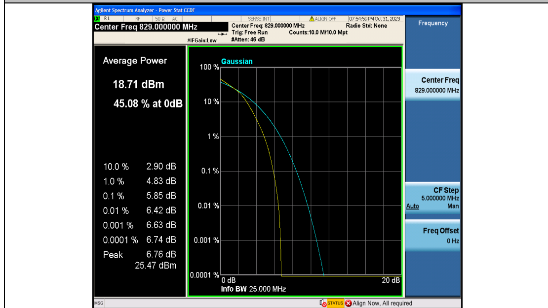
Band5-10MHz-16QAM-20450-50RB#0-PASS
