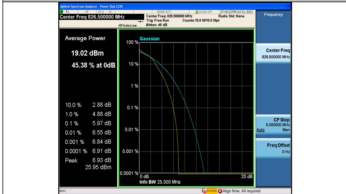
Band5-5MHz-16QAM-20425-25RB#0-PASS
