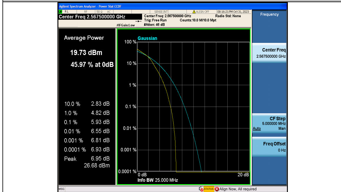
Band7-5MHz-16QAM-21425-25RB#0-PASS
