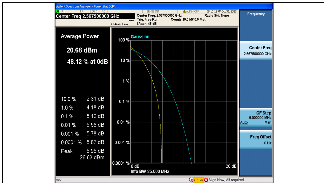
Band7-5MHz-QPSK-21425-25RB#0-PASS
