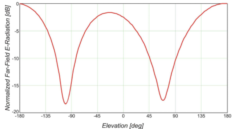
Figure 20. Normalized radiation pattern on X-Z plan (Cartesian plot)
