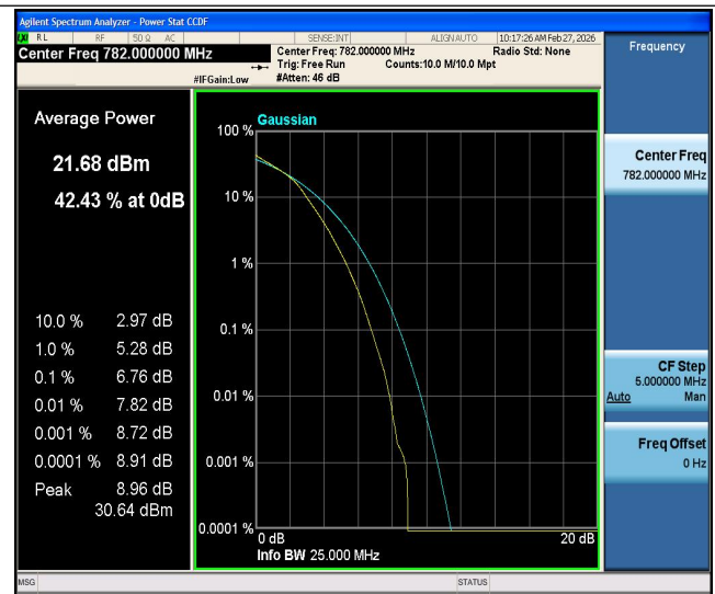
Band13-10MHz-16QAM-23230-27RB#0-PASS
