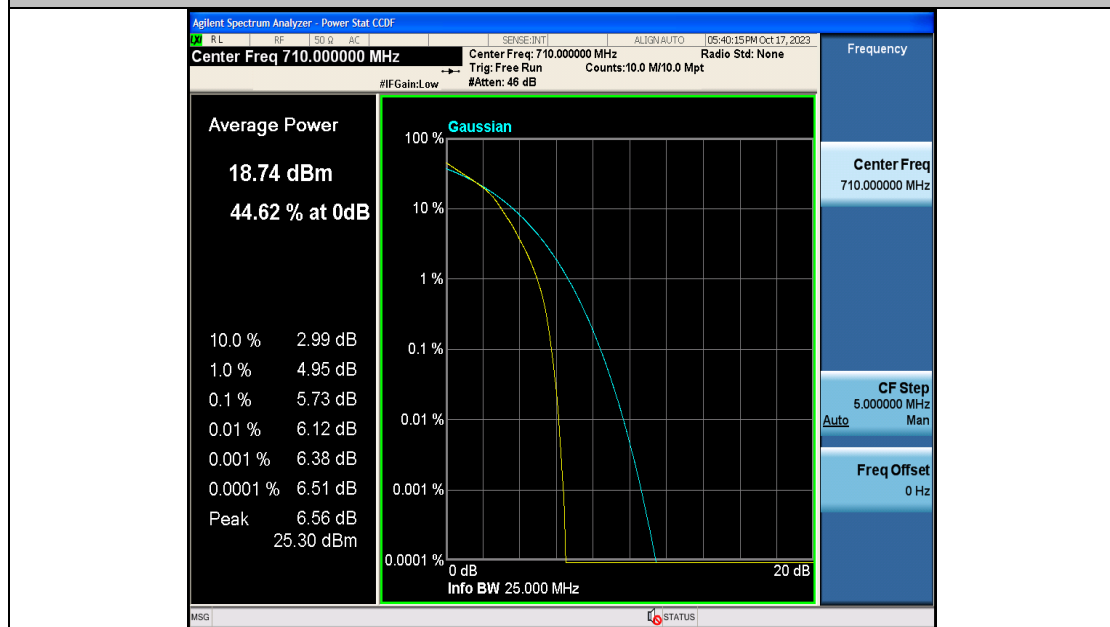
Band17-10MHz-16QAM-23790-50RB#0-PASS
