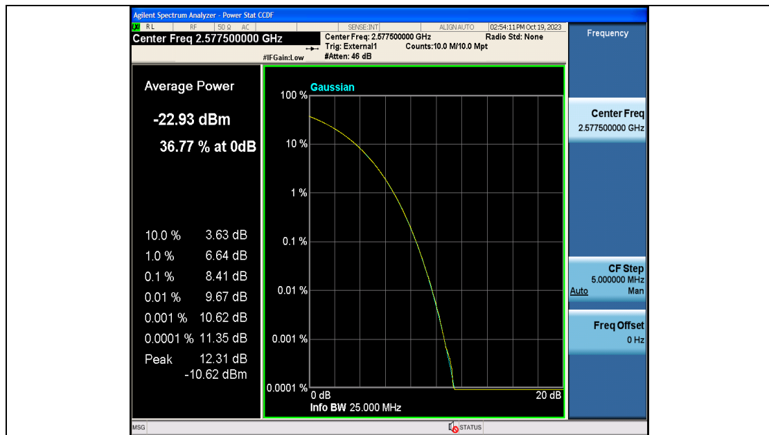
Band38-15MHz-QPSK-37825-75RB#0-PASS
