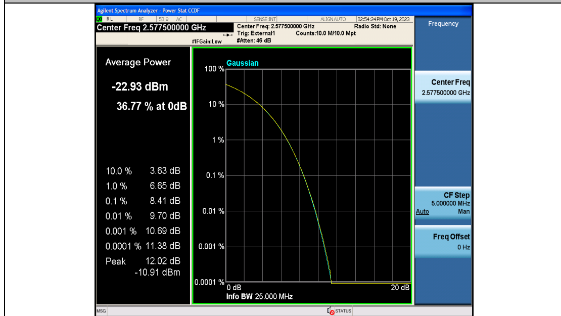
Band38-15MHz-16QAM-37825-75RB#0-PASS
