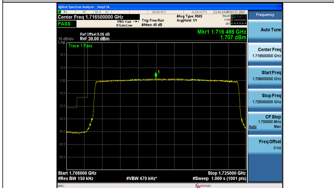
Band4_15MHz_16QAM_20025_75RB#0
