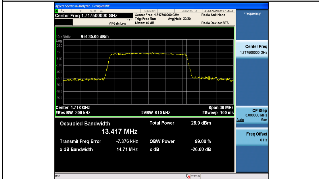
Band4-15MHz-16QAM-20025-75RB#0-PASS
