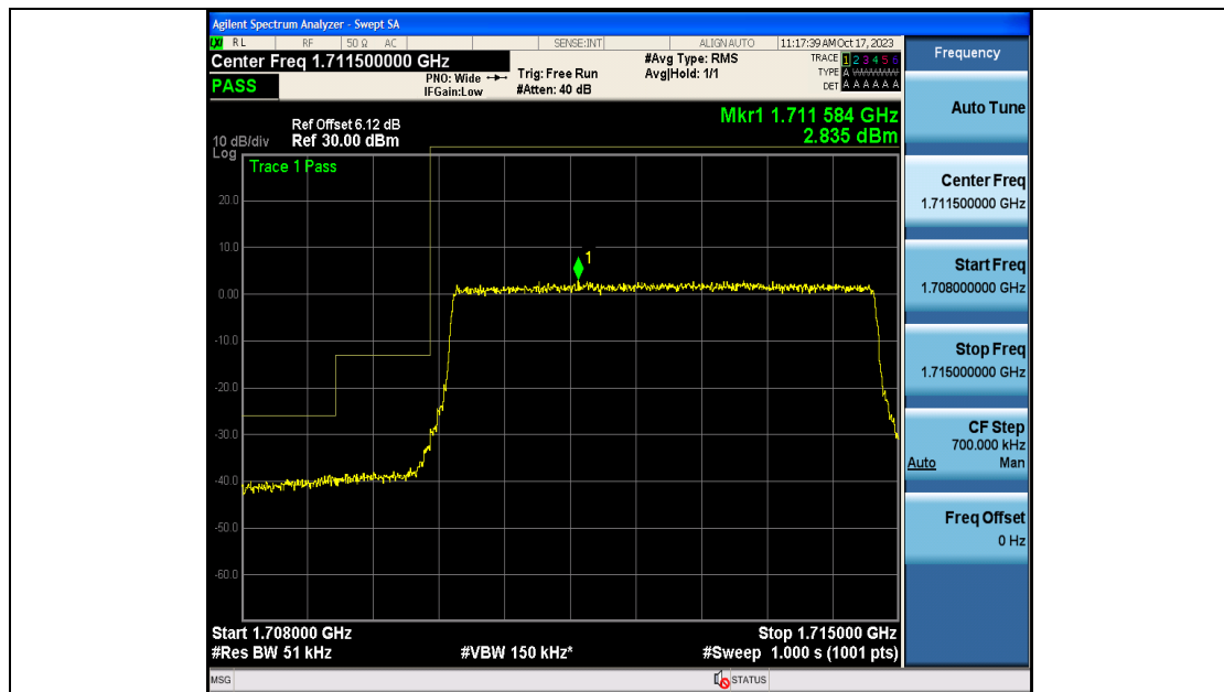
Band4_5MHz_QPSK_19975_25RB#0
