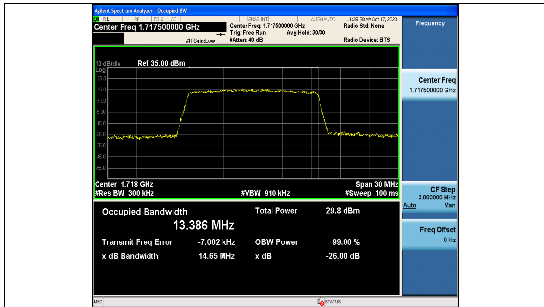
Band4-15MHz-QPSK-20025-75RB#0-PASS
