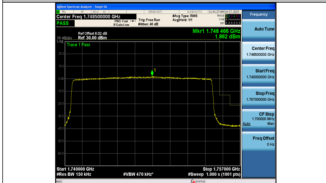
Band4_15MHz_16QAM_20325_75RB#0
