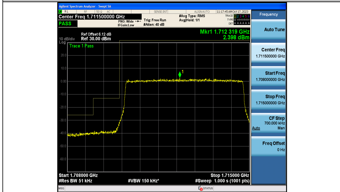
Band4_5MHz_16QAM_19975_25RB#0
