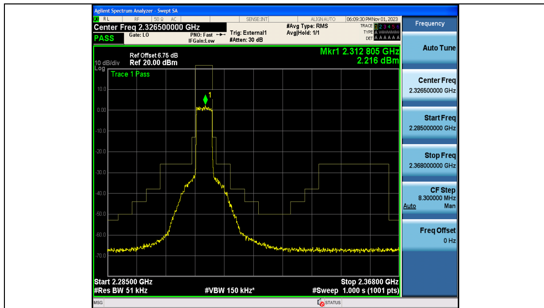
Band40_5MHz_16QAM_38775_25RB#0
