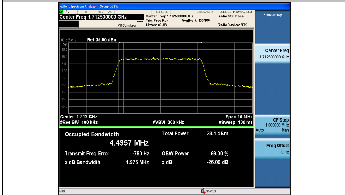
Band66-5MHz-16QAM-131997-25RB#0-PASS
