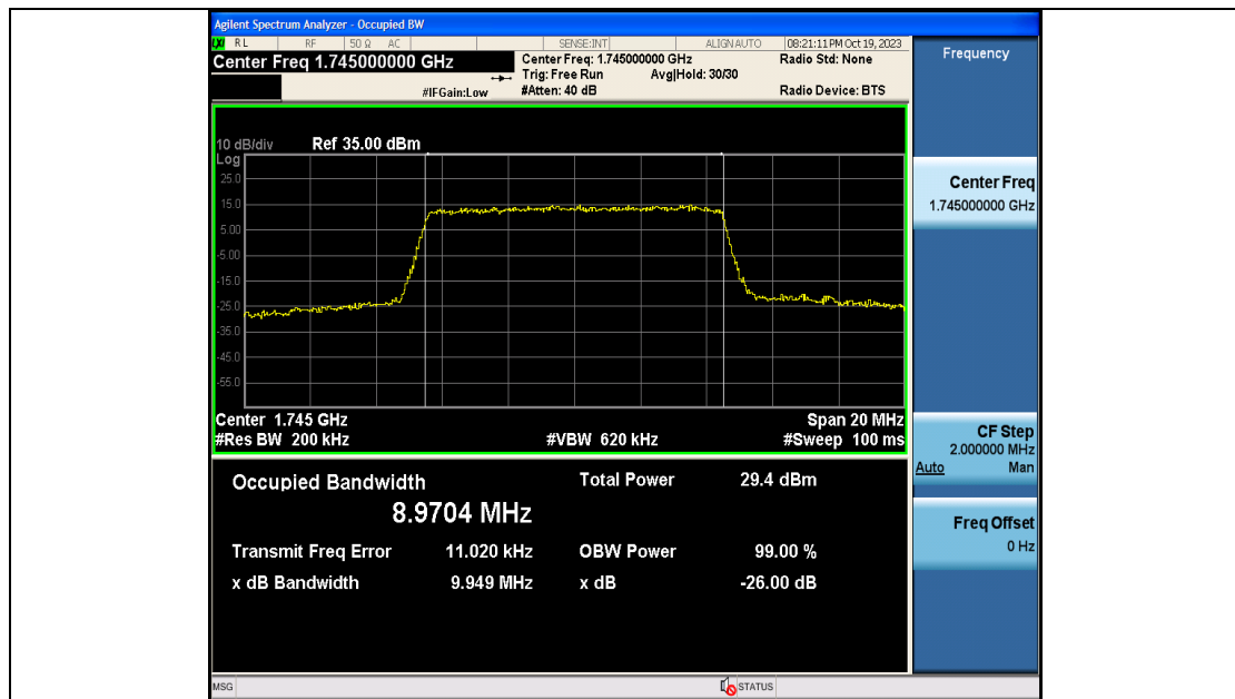
Band66-10MHz-QPSK-132322-50RB#0-PASS
