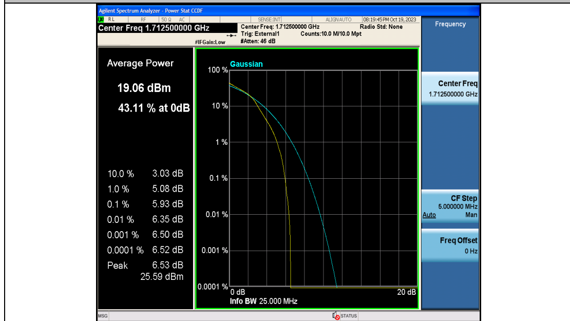
Band66-5MHz-16QAM-131997-25RB#0-PASS
