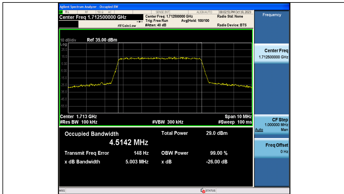
Band66-5MHz-QPSK-131997-25RB#0-PASS
