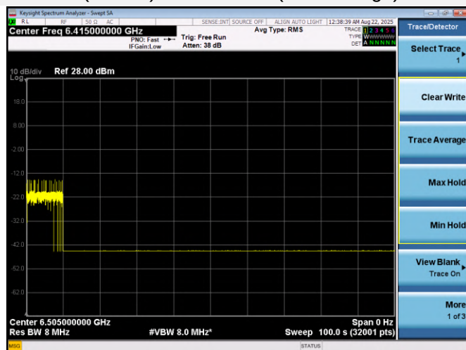
802.11ax (HE160)-Channel 111 (Middle Edge)
