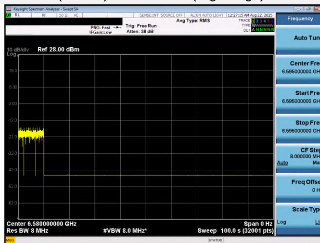
802.11ax (HE160)-Channel 111 (High Edge)
