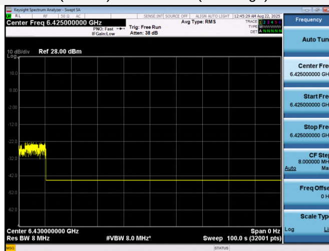
802.11ax (HE160)-Channel 111 (Low Edge)
