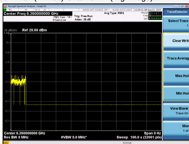
802.11ax (HE160)-Channel 47 (High Edge)
