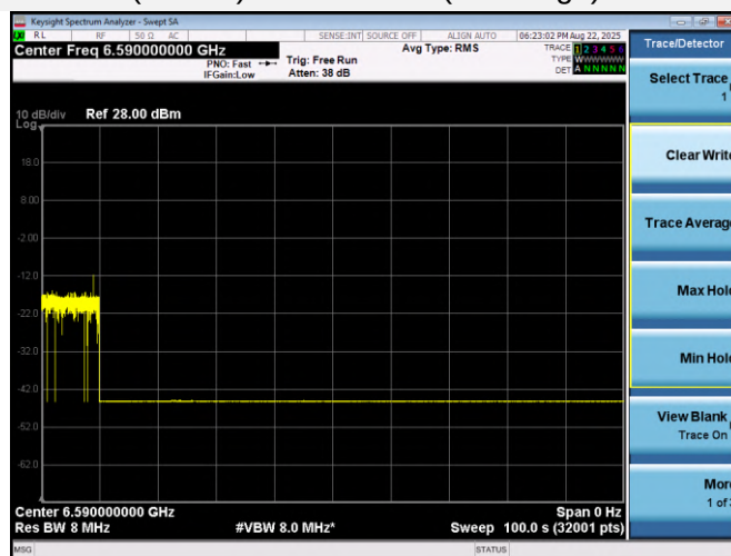
802.11ax (HE160)-Channel 143 (Low Edge)
