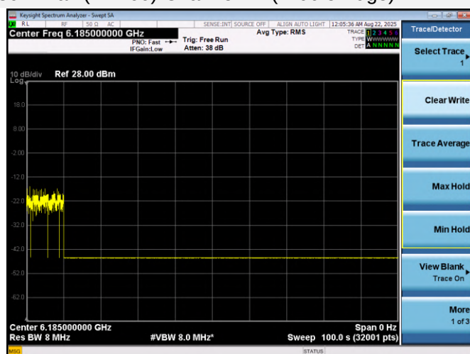
802.11ax (HE160)-Channel 47 (Middle Edge)
