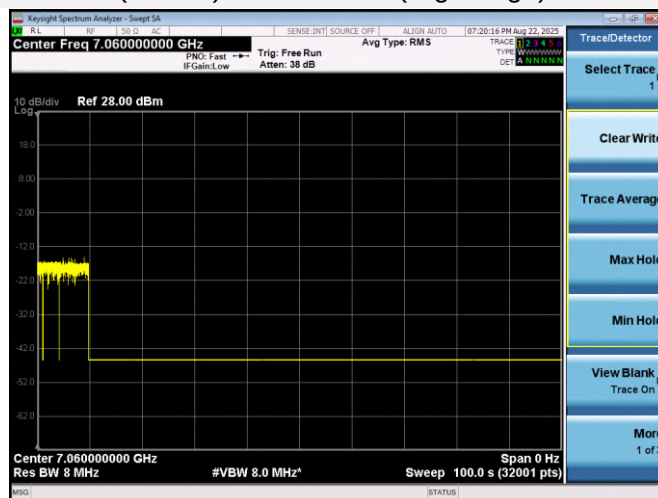
802.11ax (HE160)-Channel 207 (High Edge)
