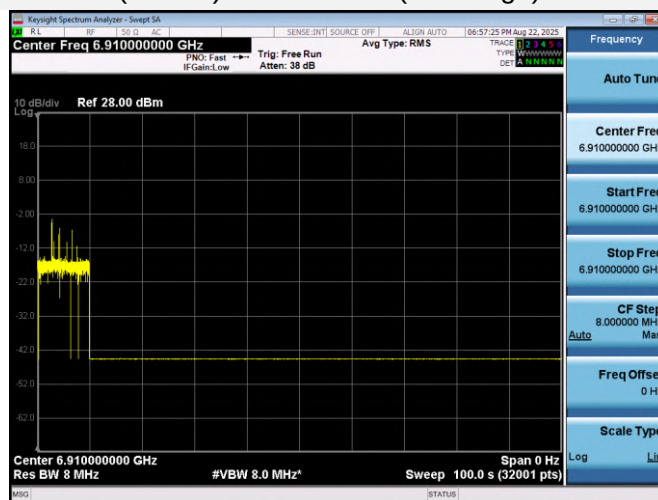
802.11ax (HE160)-Channel 207 (Low Edge)
