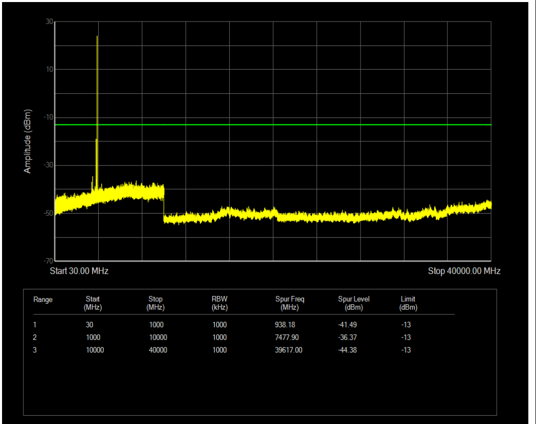
n77(3700-3980) SCS=30kHz DFT_BPSK BW=100MHz Channel=656000 RB=1@272
