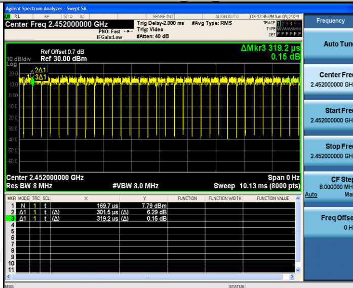
11N40SISO Ant2 2452
