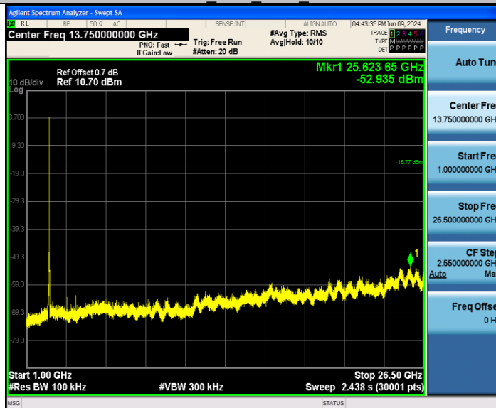
11AX20SISO Ant2 2462 1000~26500
