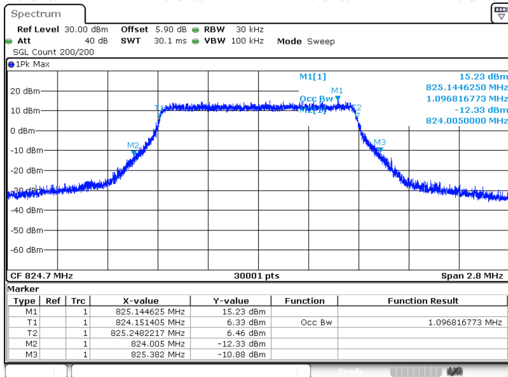
Band26(824-849) QPSK BW=1.4MHz Channel=26797 RB Size=6 Position=#0
