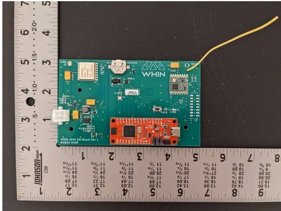
EUT Main Solder Board Top View 1
