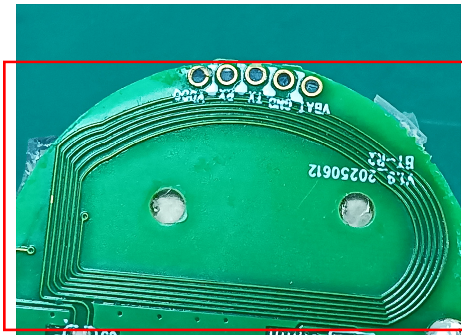
ANT-NFC(only RX)
