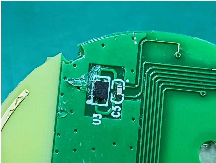
ANT-NFC(only RX)
