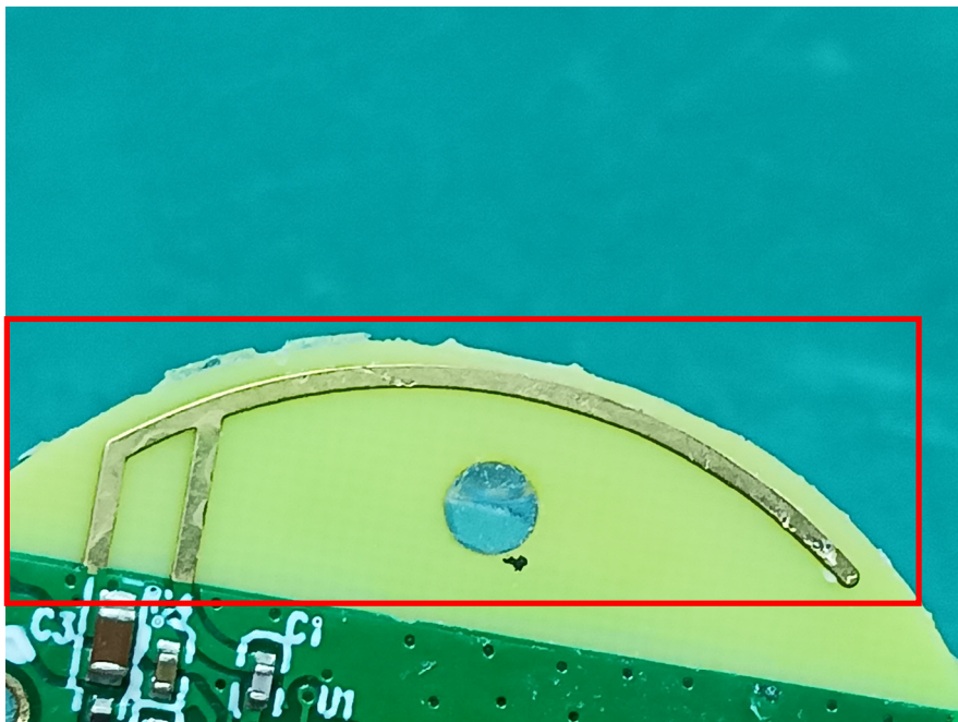
ANT-BLE
