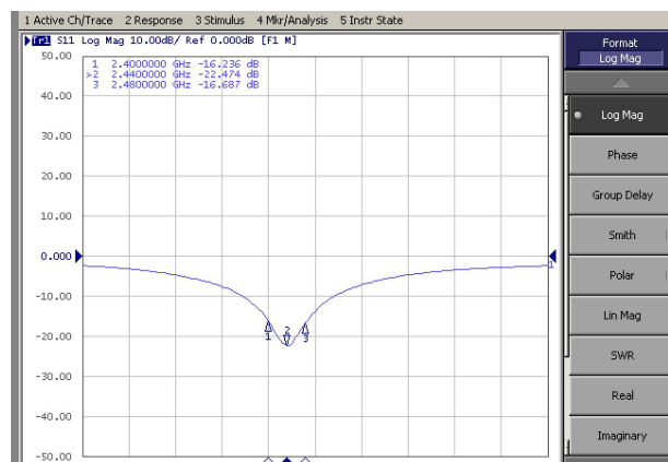
S11
