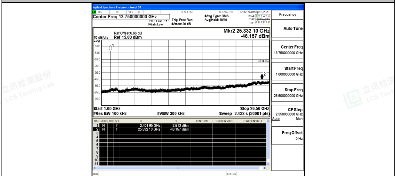
2DH5_Ant1_2441_0~Reference
