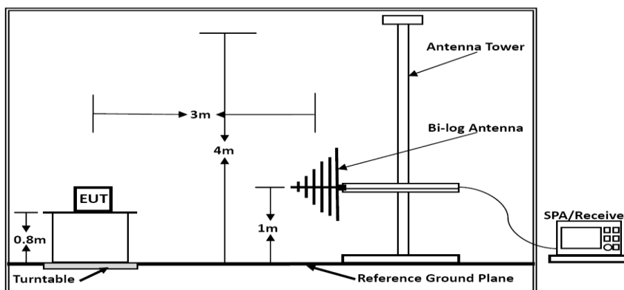
Below 1GHz
