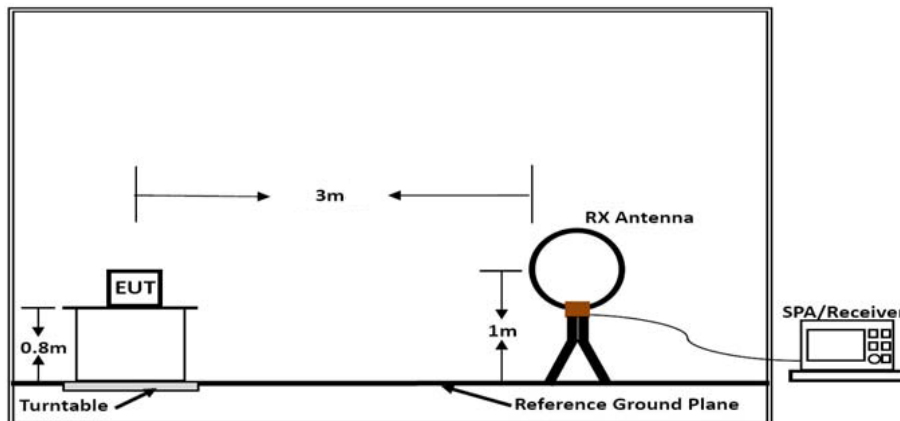
Below 30MHz
