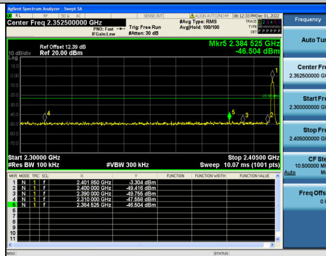
DH5-Ant1-Low-Hop_2402--3.49
