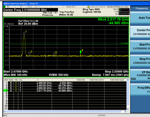
3DH5-Ant1-High-2480--2.08
