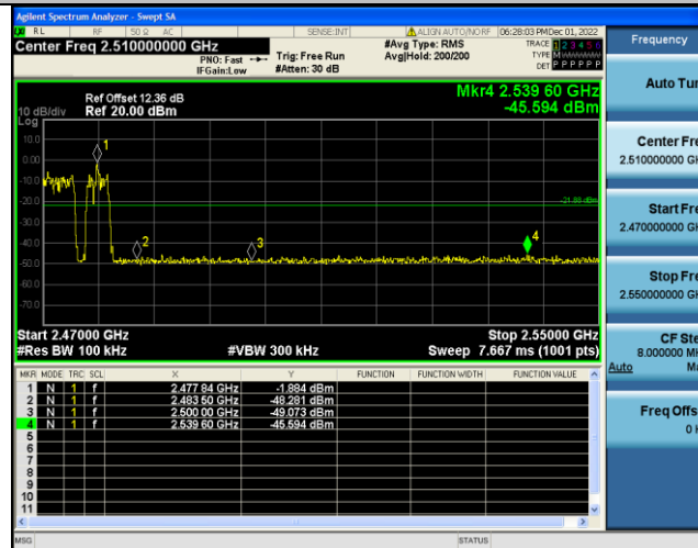
3DH5-Ant1-High-Hop_2480--1.88
