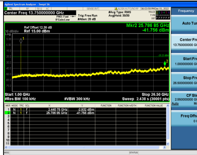
3DH5-Ant1-2441-0~Reference--6.34
