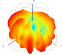
2480.0MHz H+V, Eff: 1.3%
