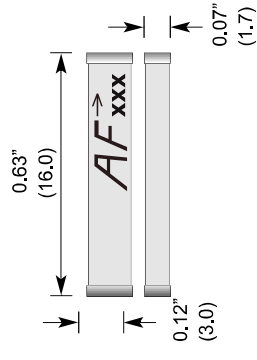
Figure 2: 868MHz and 916MHz Dimensions
