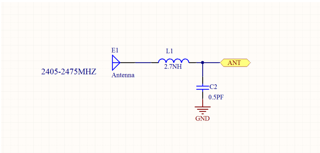
Match Network
