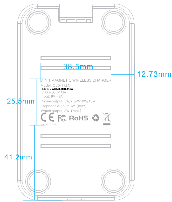
bottom cover
