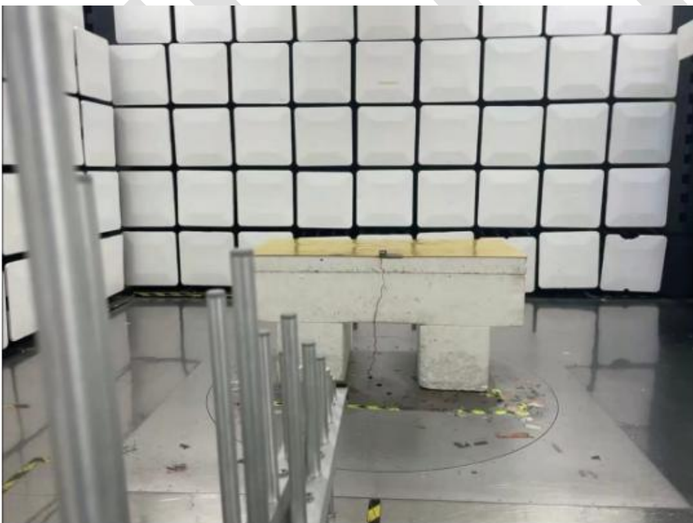
30 MHz-1 GHz Vertical
