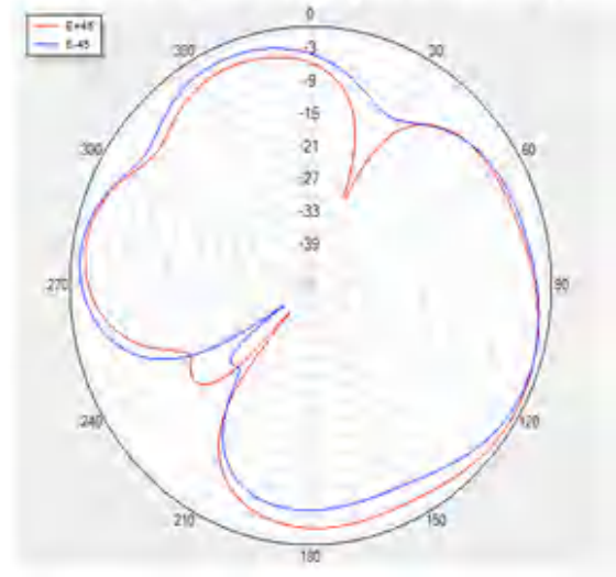
H Theta=90 freq=2450MHz
