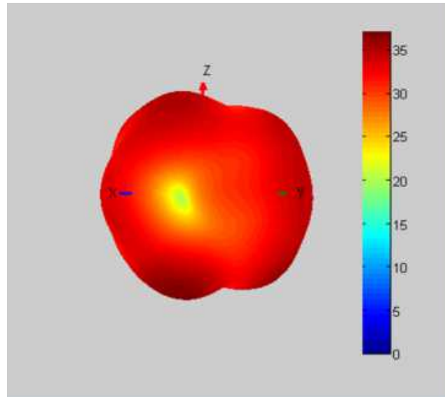
H Theta=90 freq=2480MHz
