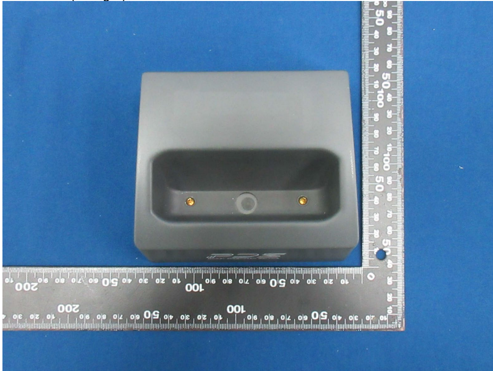
(7) EUT Photo (Charger)
