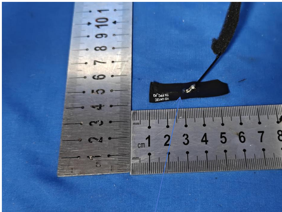
ATS2833PL FPC antenna 3.41dBi
