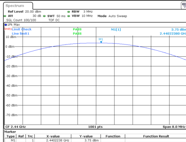
NTNV_BLE_2440_1Mbps_Peak
