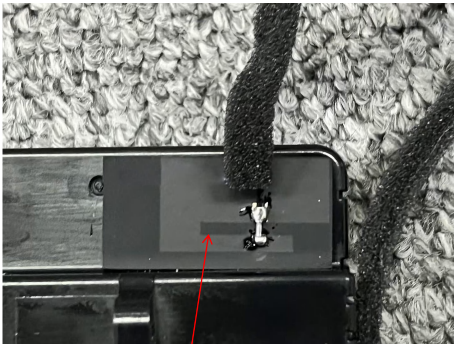
5.8G FPC Antenna gain:5dBi
