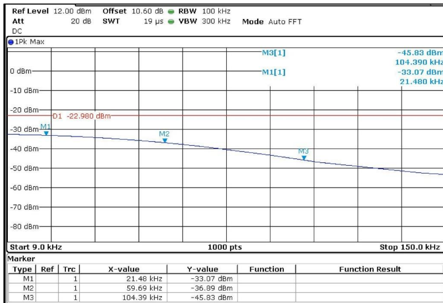
Channel Frequency 2405MHz Frequency Range 9KHz – 150KHz
