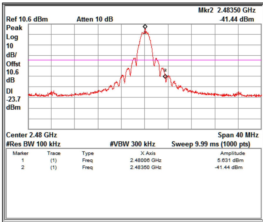
Band edge Channel Frequency 2480MHz
